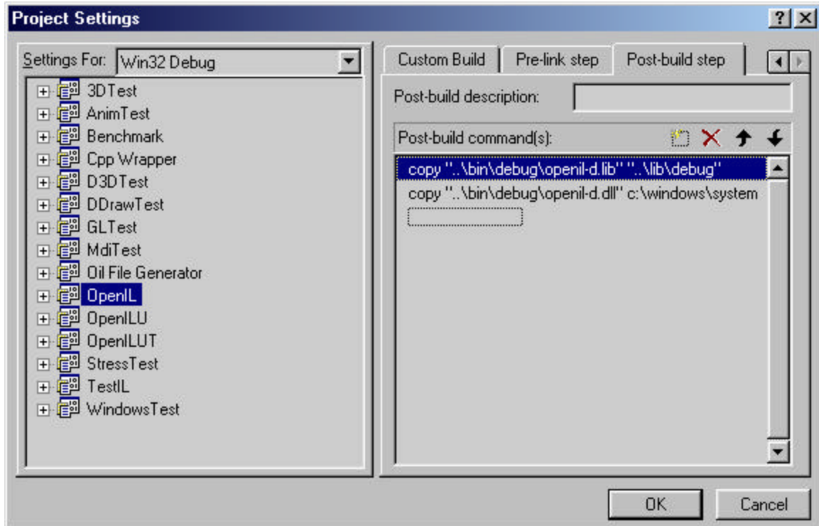
Figure 1-3. Post-Build Dialog
