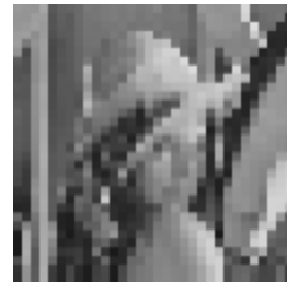
Bilinear filter
