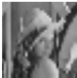
Triangle filter
